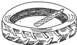
Wood ramp with strap hinge, covered with 1/2" hardware cloth. Length of ramp should be a least 18" greater than depth of tank.
